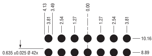
PACKAGE TOP VIEW
