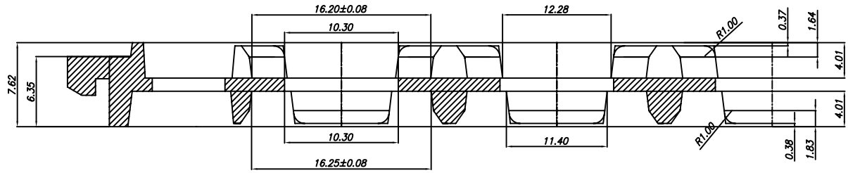
SECTION "A-A" (SCALE:5/1)
