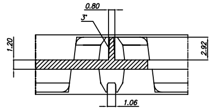
VACUUM CELL (SCALE:5/1)
