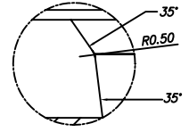
DETAIL "G" (SCALE:12/1)
