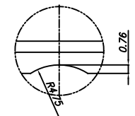
DETAIL "K" (SCALE:4/1)
