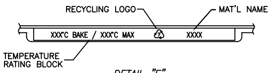
DETAIL "F" (SCALE:2/1)
