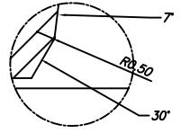
DETAIL "H" (SCALE:12/1)
