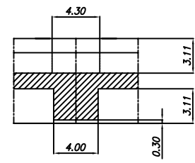
SLIP LOCK (SCALE:5/1)
