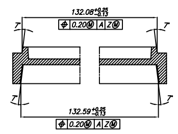
TRAY STACKING DETAIL (SCALE:4/1)
