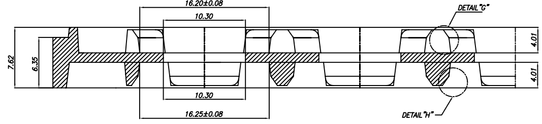
SECTION "A-A" (SCALE:5/1)
