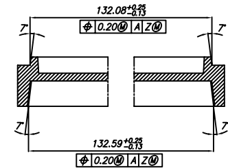
TRAY STACKING DETAIL (SCALE:4/1)
