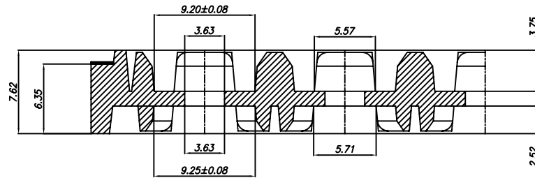
SECTION "A-A" (SCALE:5/1)
