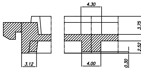
SLIP LOCK (SCALE:5/1)
