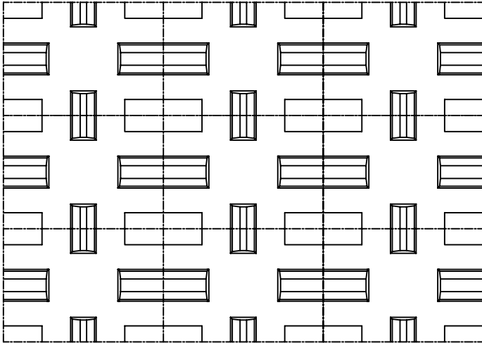
TOP VIEW (SCALE:4/1)
