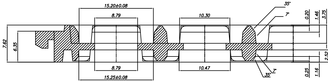
SECTION "A-A" (SCALE:5/1)
