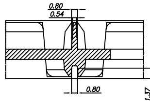
VACUUM DETAIL (SCALE:5/1)
