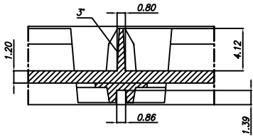
VACUUM CELL (SCALE:5/1)
