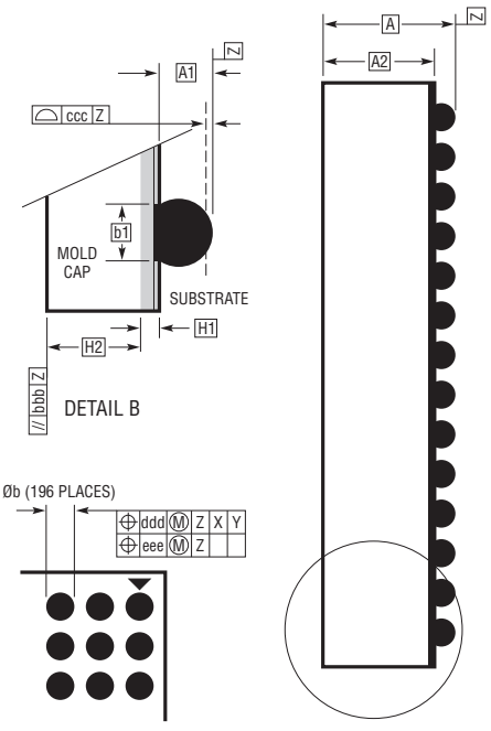
DETAIL B PACKAGE SIDE VIEW
