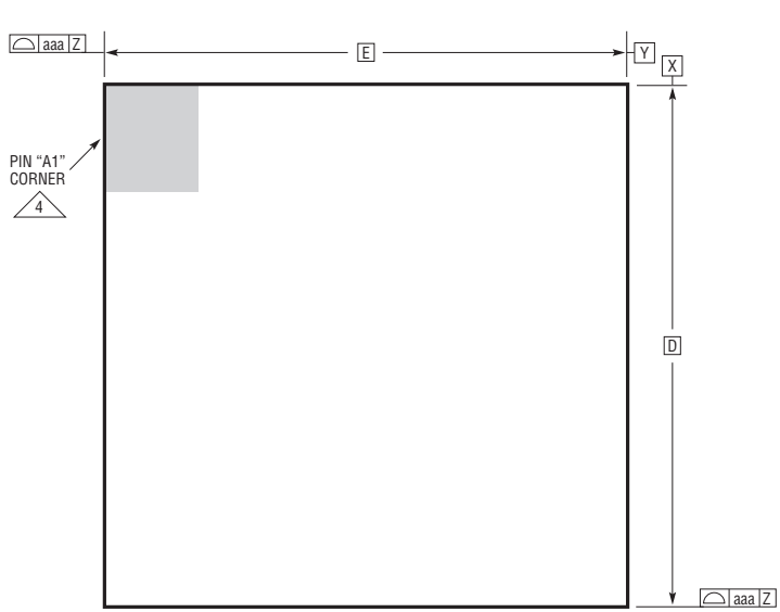
PACKAGE TOP VIEW
