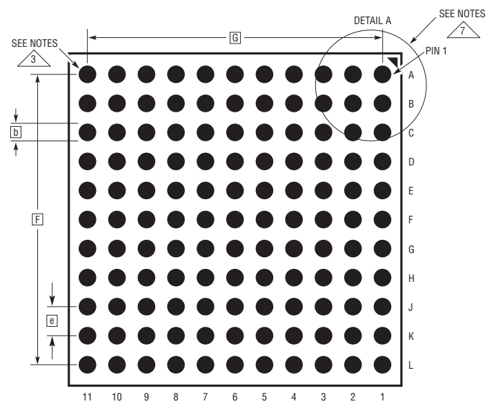
PACKAGE BOTTOM VIEW
