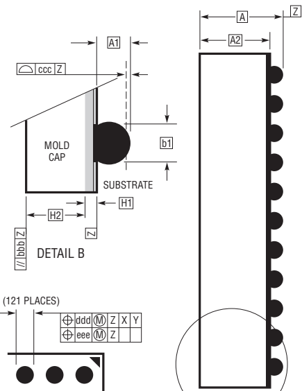
DETAIL B PACKAGE SIDE VIEW
