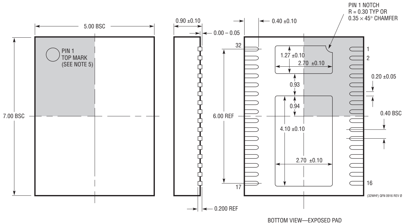
BOTTOM VIEW—EXPOSED PAD
