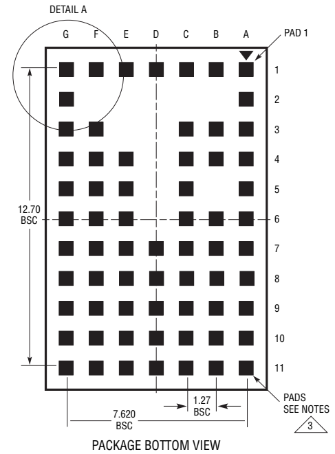
PACKAGE BOTTOM VIEW
