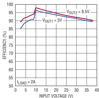
Figure 2. Efficiency vs input voltage for Figure 1.
