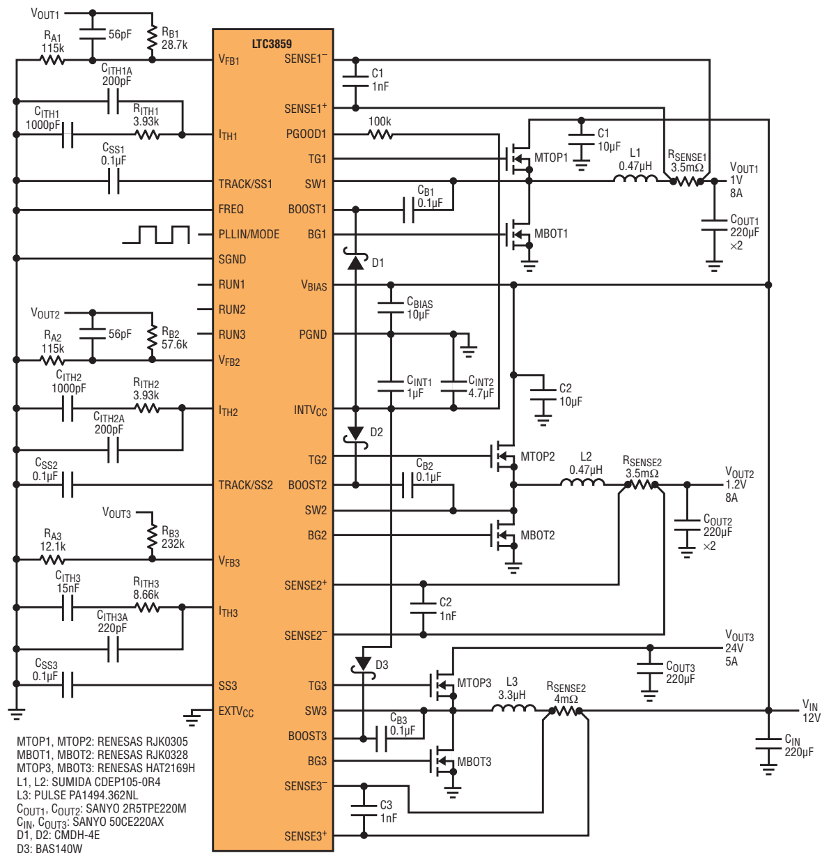
Figure 4. General purpose triple output application using the LTC3859
