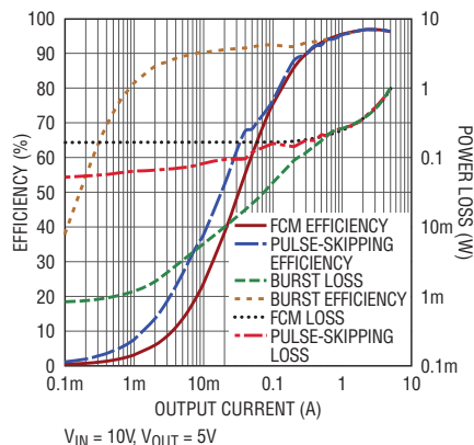
Figure 3. Efficiency and power loss vs load current of 5V output for Figure 1.
