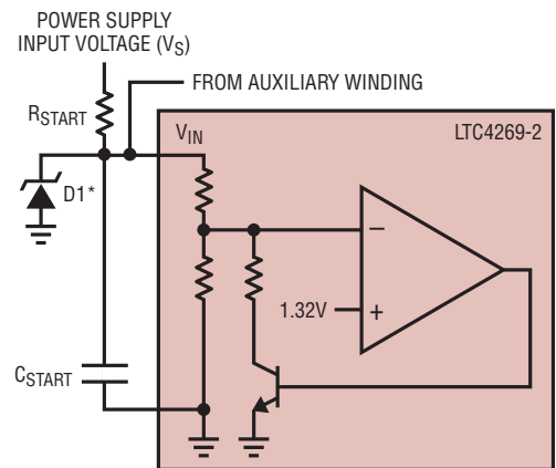
Figure 9. Programming Power Supply Undervoltage Lockout (UVLO)
