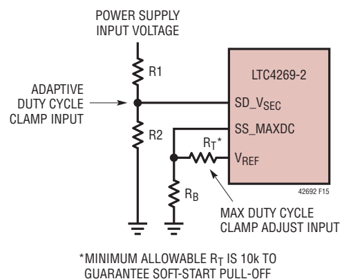
Figure 15. Programming Maximum Duty Cycle Clamp
