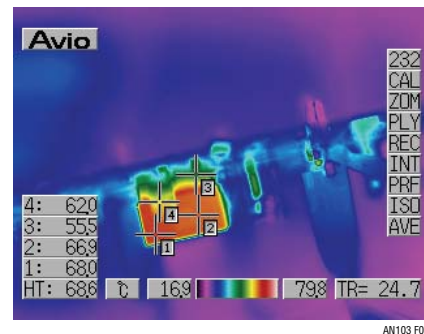
CONDITIONS: 25°C, NO AIR FLOW, WAKEFIELD ENGINEERING PN# 20069, 15mm \times 15mm \times 9mm HEATSINK, NO EXT V CC
